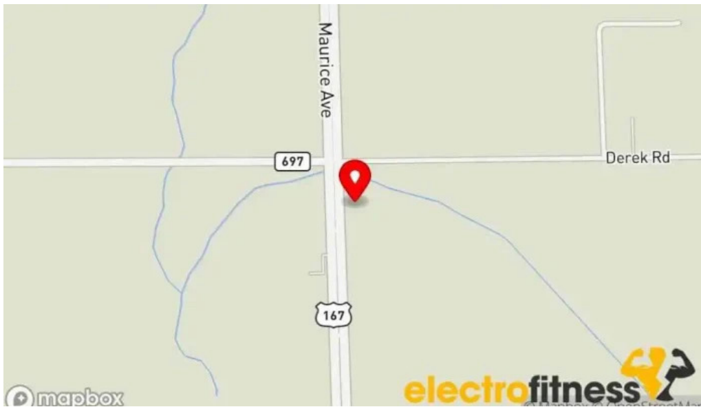
Vermilion crossfit map
